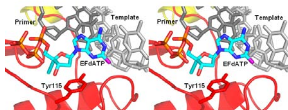
Figure 4. Stereo view of EFdATP (cyan) modeled in the RT active site. The 3'-OH of EFdATP is in the North conformation and is free of steric interactions with Tyr115 (red sticks). The primer is in dark gray, the template in light gray, the connection subdomain in yellow, and the palm subdomain in red. The fingers subdomain was removed for clarity. Image generated using PyMOL (7).
