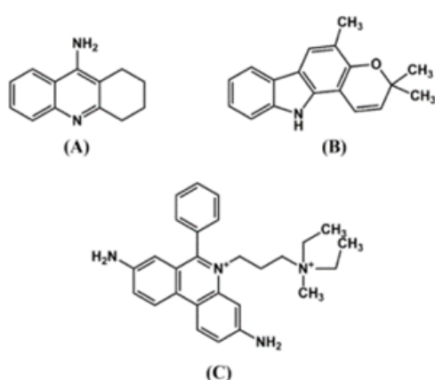
Fig. 1. 2D structures of Tacrine (A), Grinimbine (B), and Propidium (C).
